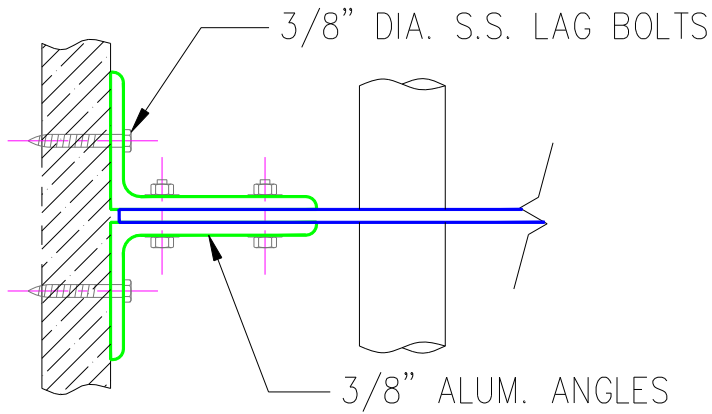
STANDARD MOUNTING ~ TOP VIEW (ALTERNATE MOUNTING STYLES AVAILABLE)
